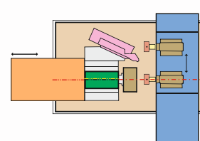
TWO AXIS TWO SPINDLE
