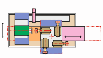
FIVE AXIS FOUR SPINDLE
